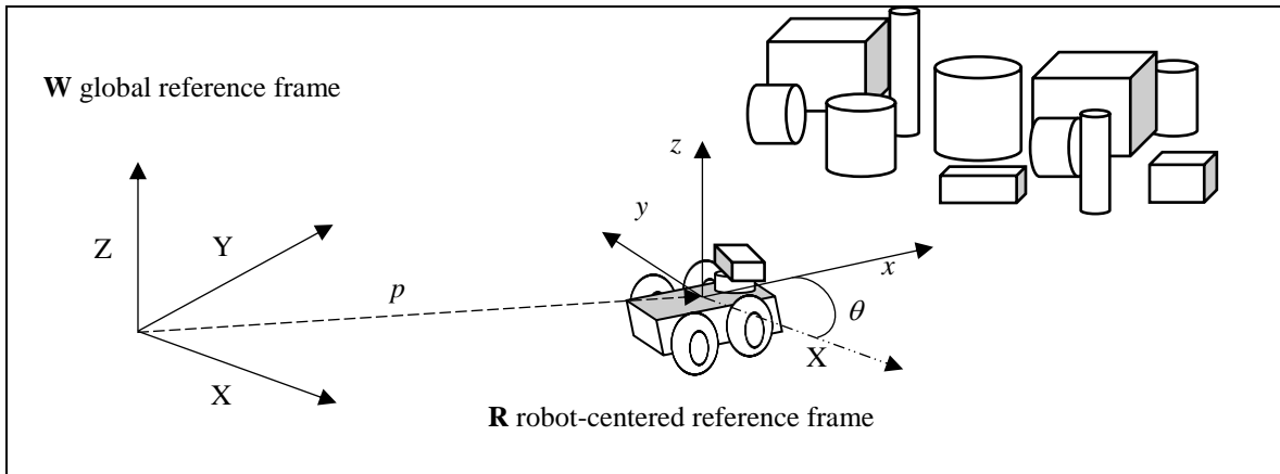
Figure 1: Summary of coordinate frames for an HSV homing mission.
