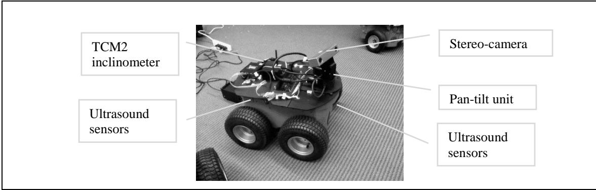
Figure 4: Pioneer 3AT with Bumbleb2 stereo-camera on Dynamic Perception Pan-Tilt unit and TCM2 inclinometer.
