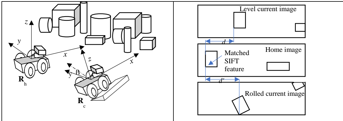
Figure 3: (a) Summary of coordinate frames on uneven terrain for an HSV homing mission. (b) Homing without knowledge of roll angle showing erroneous matched feature distance d' > d .
